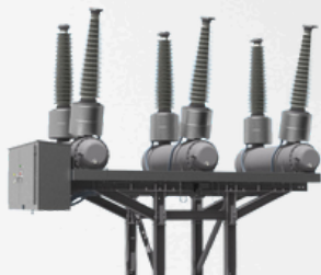
DTI-I45R-40 72.5/123/145 kV
